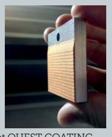
Dense deposit (porosity <0.2%) of copper produced by Cold Spray at OUEST COATING
